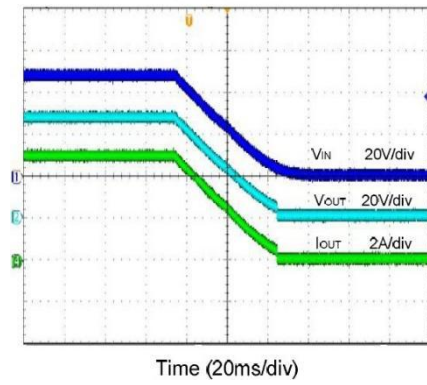
Shutdown from V_{IN} ( V_{IN}=48V, I_o=5A )
